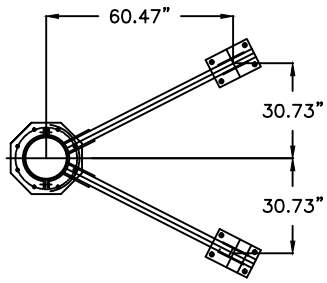
PLAN VIEW (4.5M ON KINGPOST WITH REAR KICKERS)
